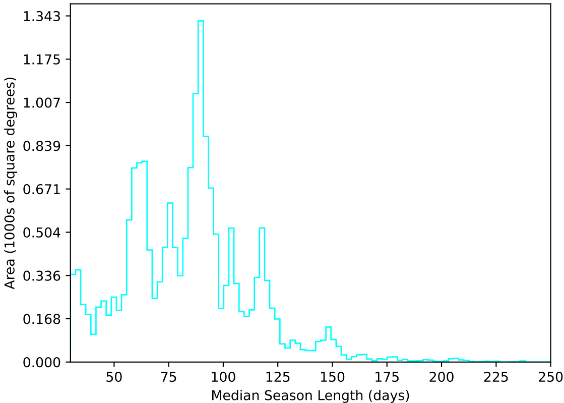
weather_cloudso31v3.4_10yrs WFD u band: Median Season Length
