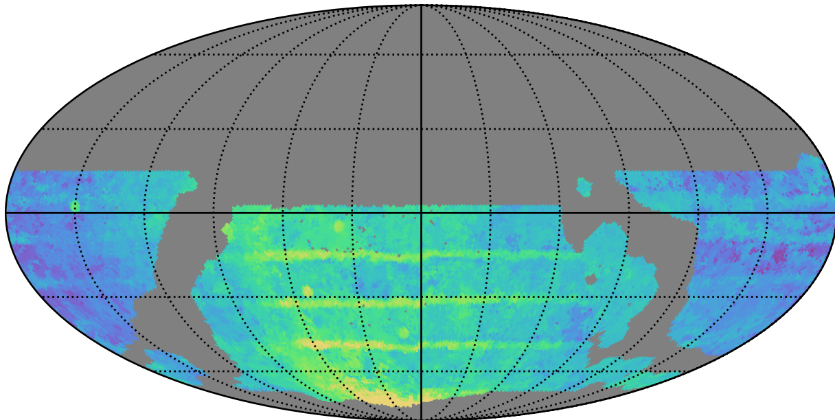
weather_cloudso31v3.4_10yrs WFD r band: Median Season Length
