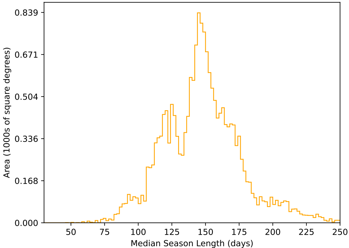
weather_cloudso31v3.4_10yrs WFD r band: Median Season Length
