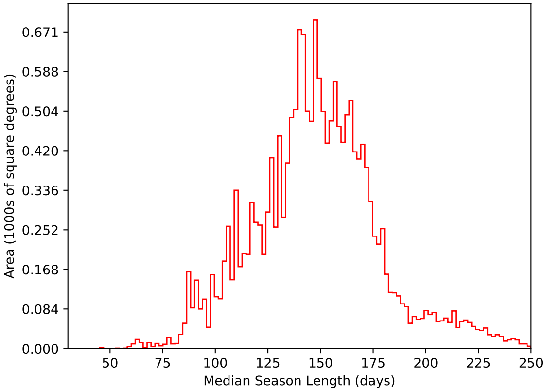
weather_cloudso31v3.4_10yrs WFD i band: Median Season Length
