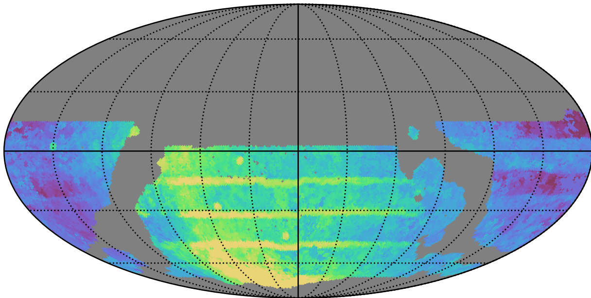
weather_cloudso31v3.4_10yrs WFD all bands: Median Season Length
