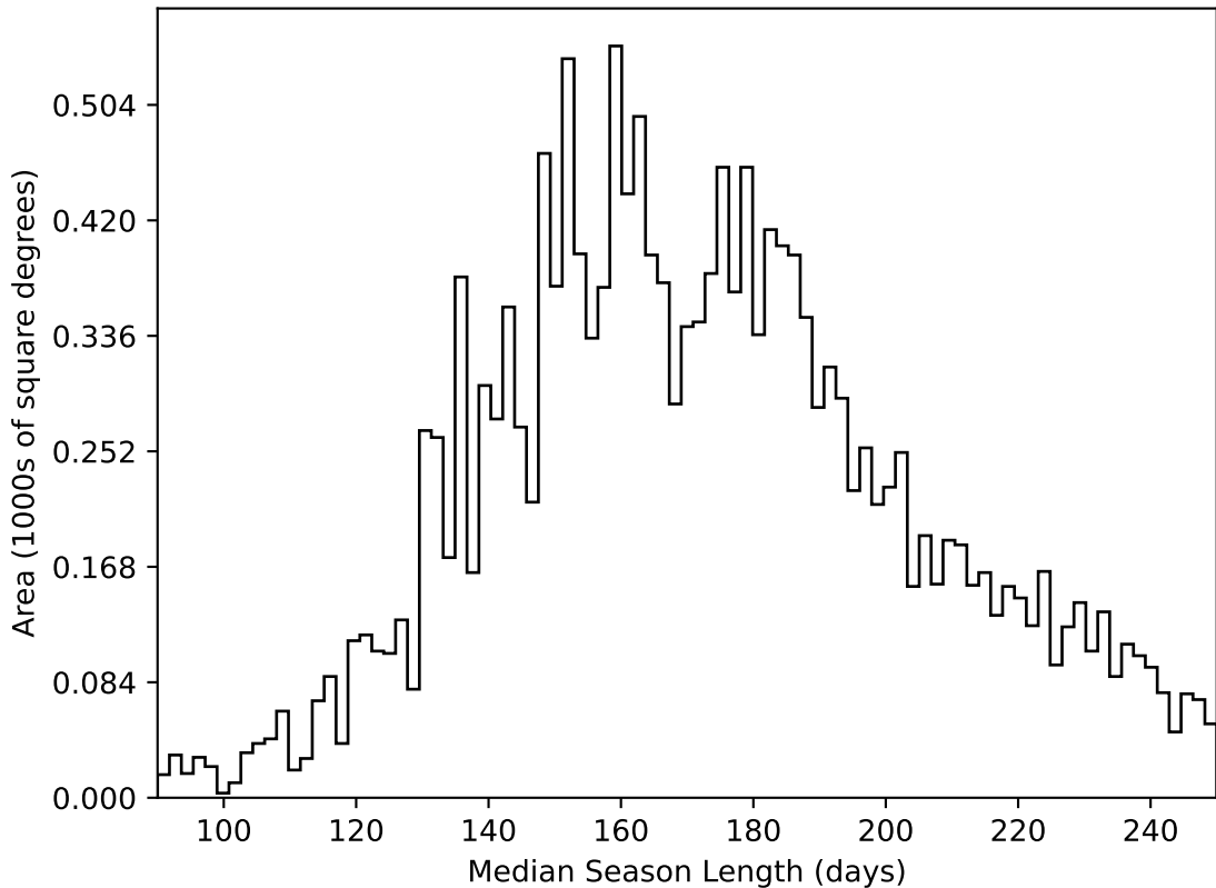
weather_cloudso31v3.4_10yrs WFD all bands: Median Season Length
