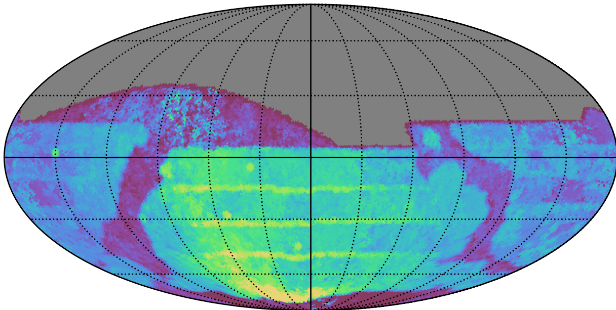
weather_cloudso31v3.4_10yrs All sky z band: Median Season Length
