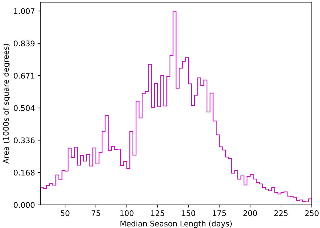
weather_cloudso31v3.4_10yrs All sky z band: Median Season Length
