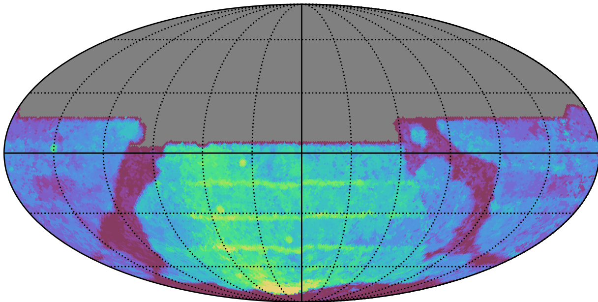
weather_cloudso31v3.4_10yrs All sky y band: Median Season Length
