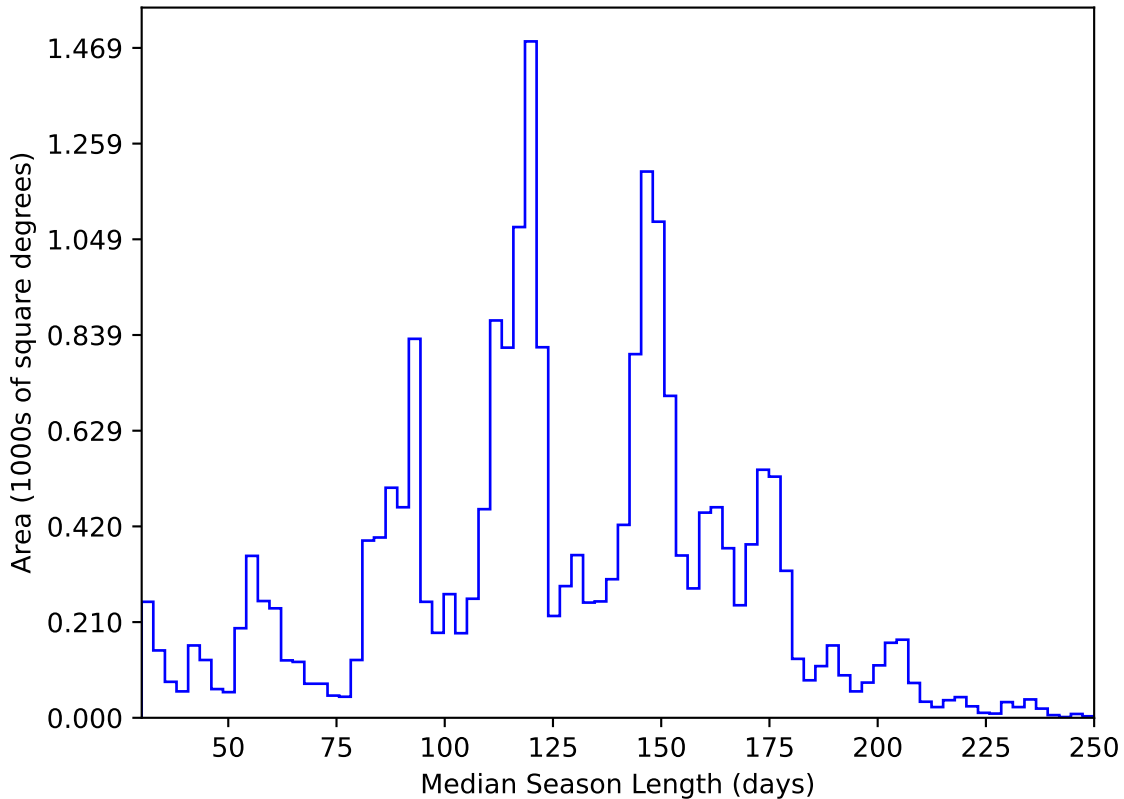
weather_cloudso31v3.4_10yrs All sky y band: Median Season Length
