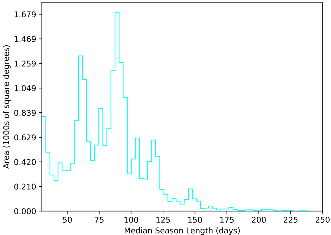
weather_cloudso31v3.4_10yrs All sky u band: Median Season Length
