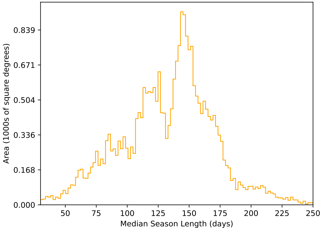
weather_cloudso31v3.4_10yrs All sky r band: Median Season Length
