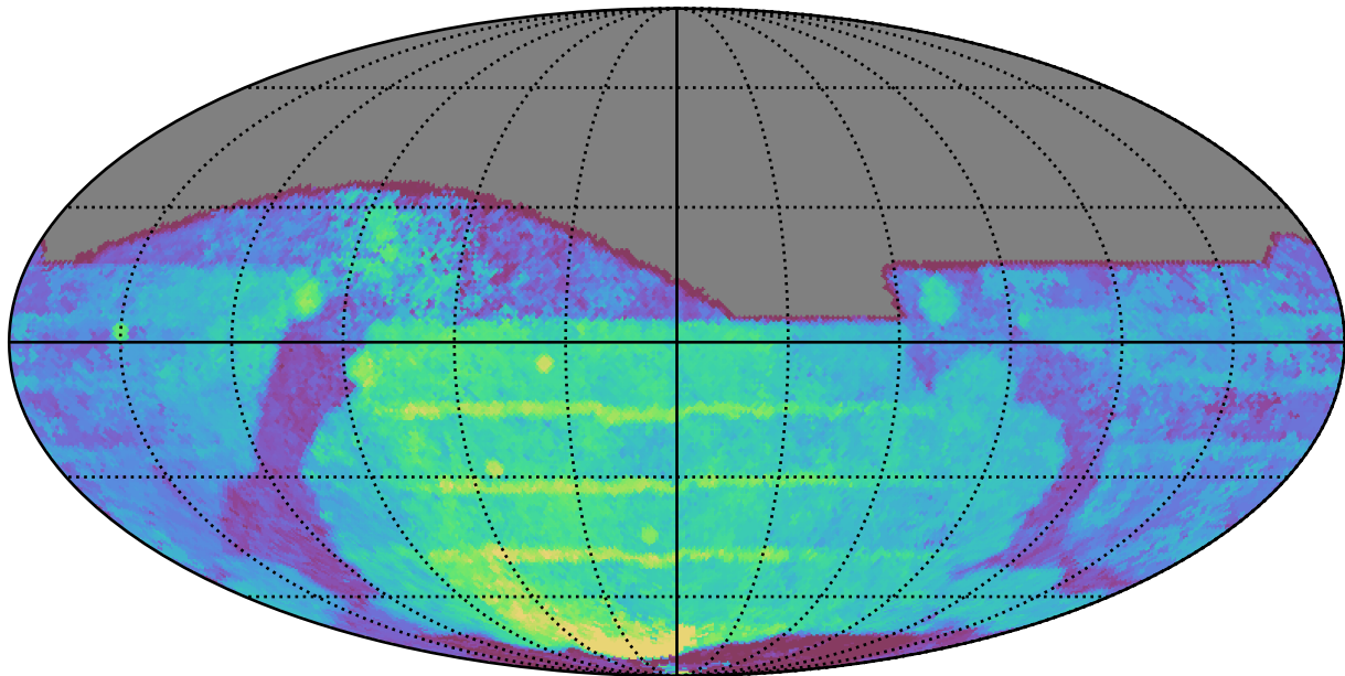
weather_cloudso31v3.4_10yrs All sky i band: Median Season Length
