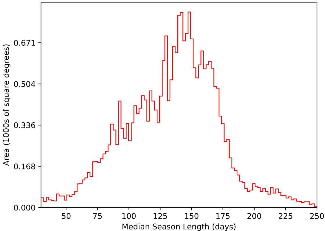
weather_cloudso31v3.4_10yrs All sky i band: Median Season Length
