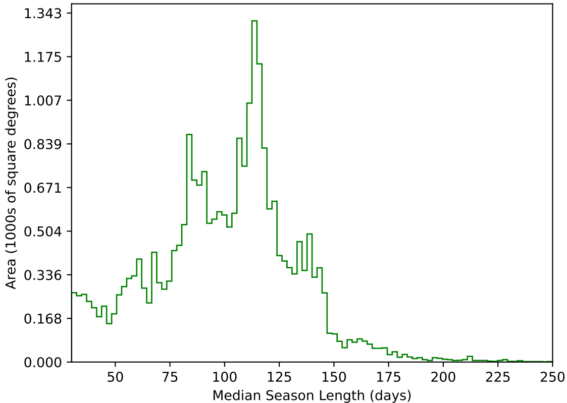
weather_cloudso31v3.4_10yrs All sky g band: Median Season Length
