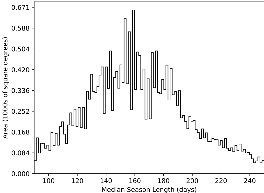
weather_cloudso31v3.4_10yrs All sky all bands: Median Season Length
