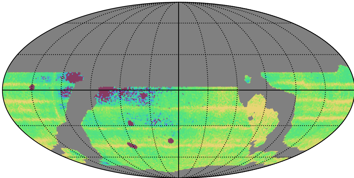
weather_cloudso31v3.4_10yrs WFD: Median Intra-Night Gap
