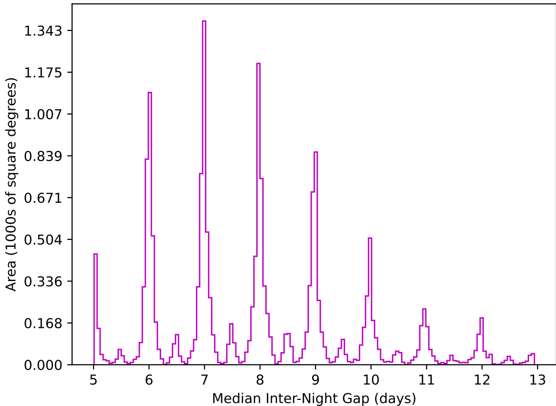
weather_cloudso31v3.4_10yrs WFD z band: Median Inter-Night Gap
