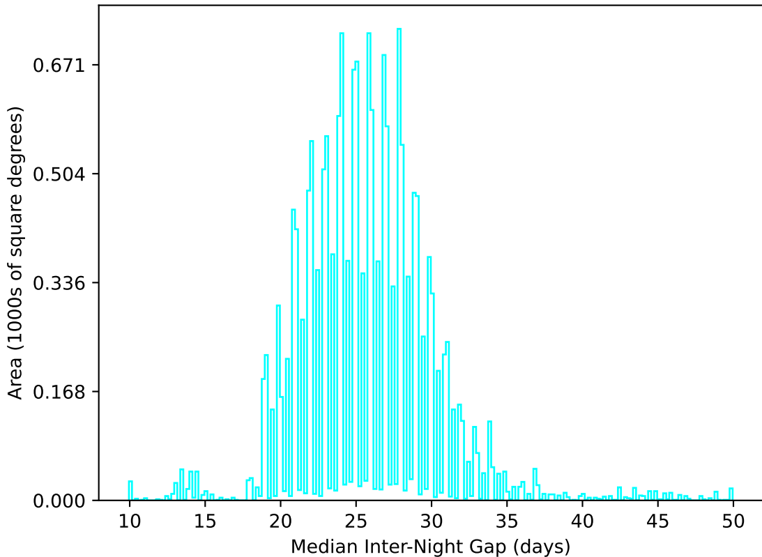
weather_cloudso31v3.4_10yrs WFD u band: Median Inter-Night Gap
