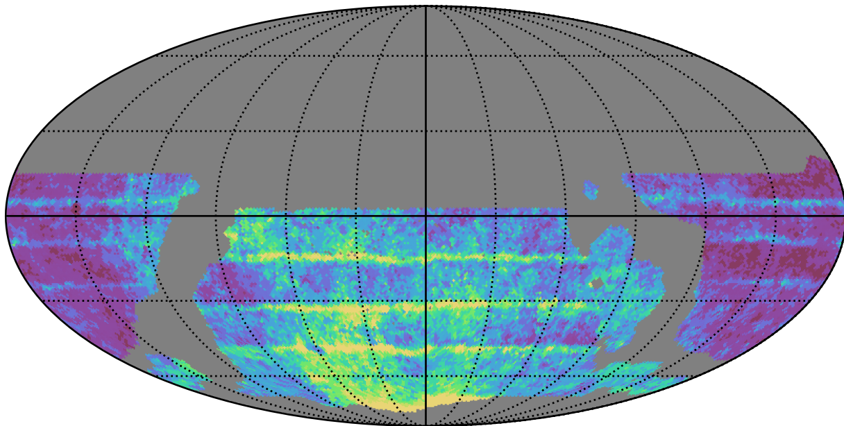
weather_cloudso31v3.4_10yrs WFD r band: Median Inter-Night Gap
