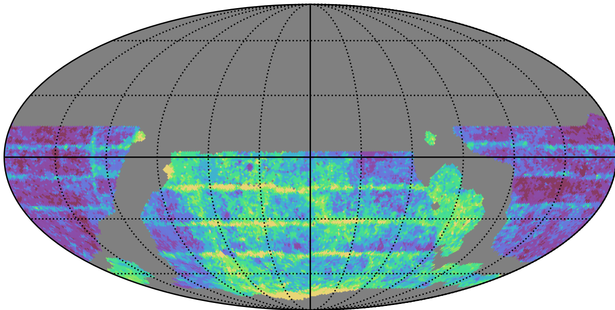
weather_cloudso31v3.4_10yrs WFD i band: Median Inter-Night Gap
