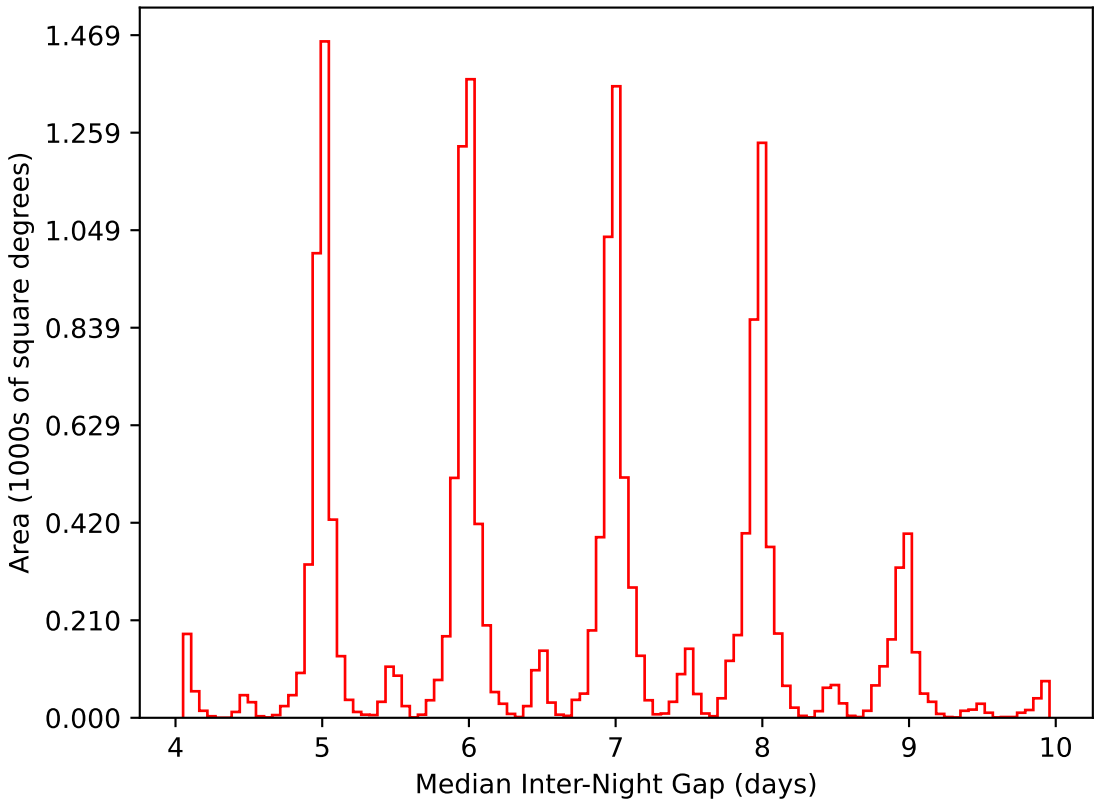
weather_cloudso31v3.4_10yrs WFD i band: Median Inter-Night Gap
