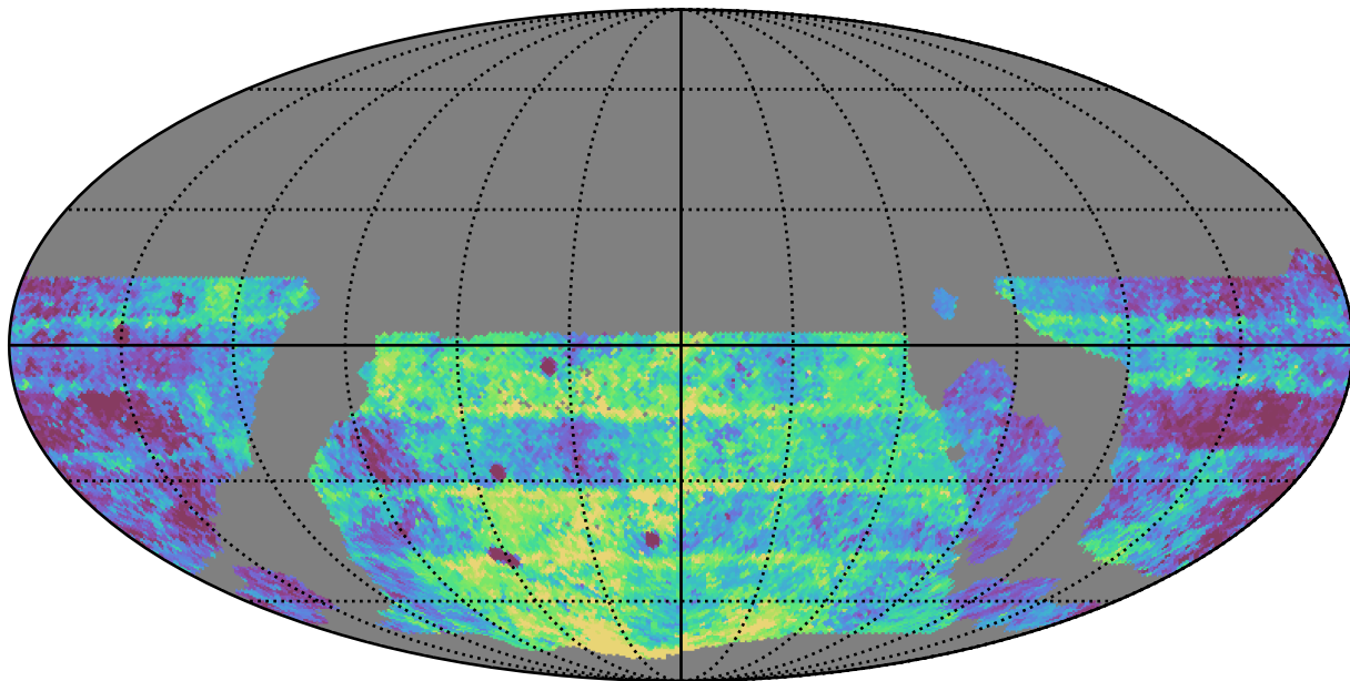
weather_cloudso31v3.4_10yrs WFD g band: Median Inter-Night Gap
