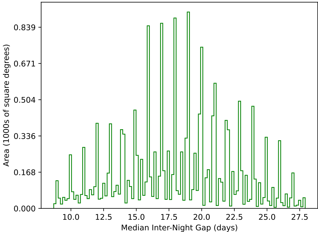
weather_cloudso31v3.4_10yrs WFD g band: Median Inter-Night Gap
