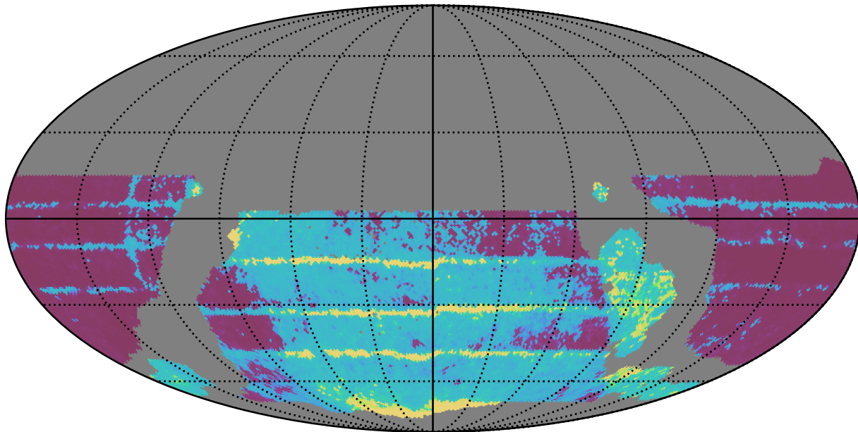
weather_cloudso31v3.4_10yrs WFD all bands: Median Inter-Night Gap
