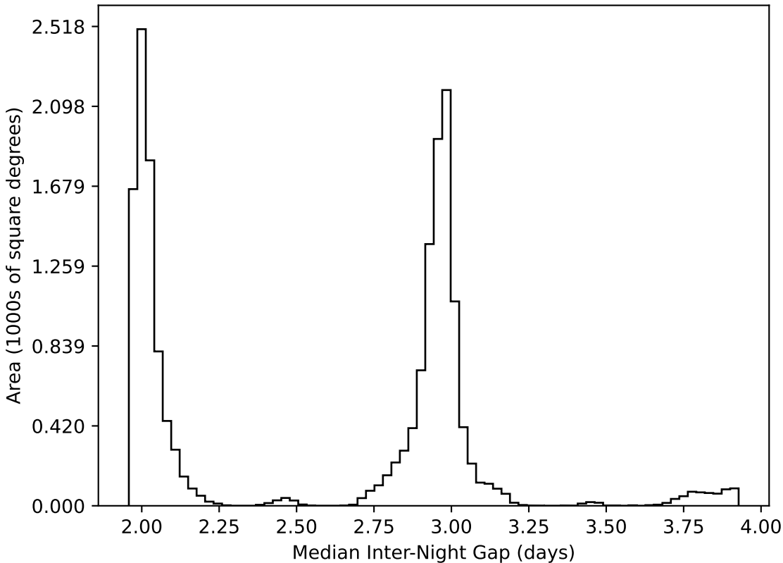
weather_cloudso31v3.4_10yrs WFD all bands: Median Inter-Night Gap
