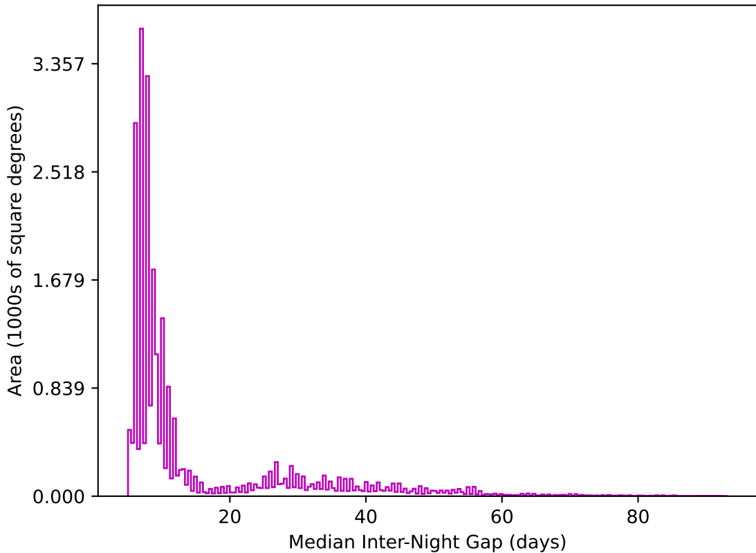
weather_cloudso31v3.4_10yrs All sky z band: Median Inter-Night Gap
