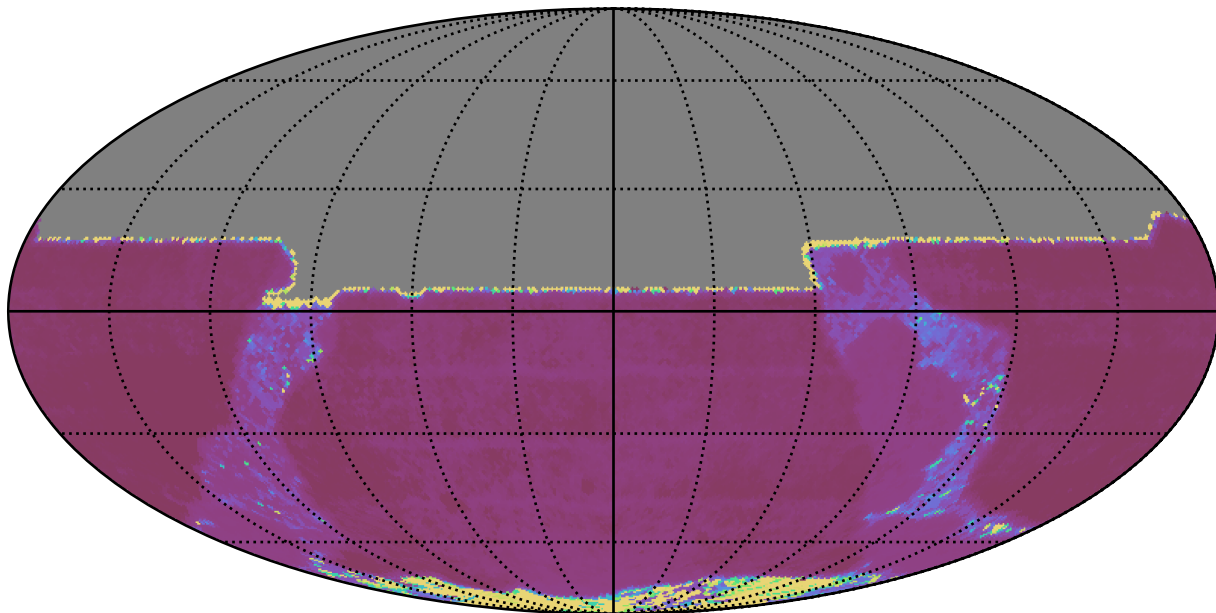
weather_cloudso31v3.4_10yrs All sky y band: Median Inter-Night Gap
