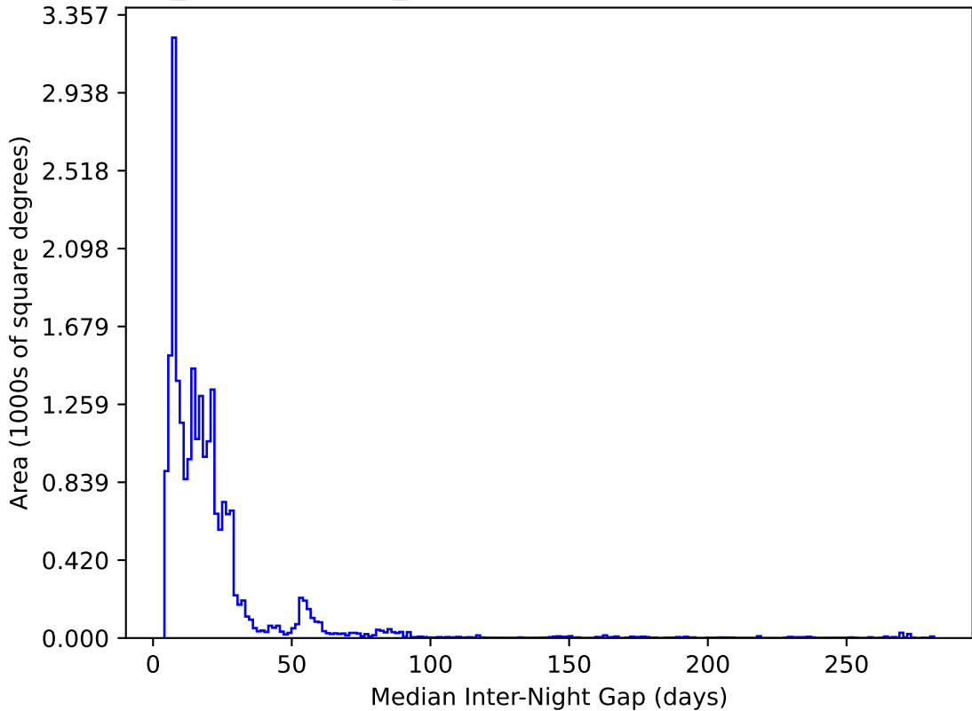
weather_cloudso31v3.4_10yrs All sky y band: Median Inter-Night Gap
