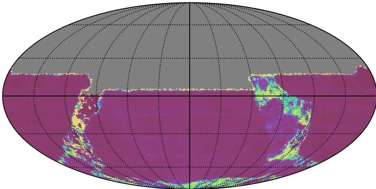
weather_cloudso31v3.4_10yrs All sky u band: Median Inter-Night Gap
