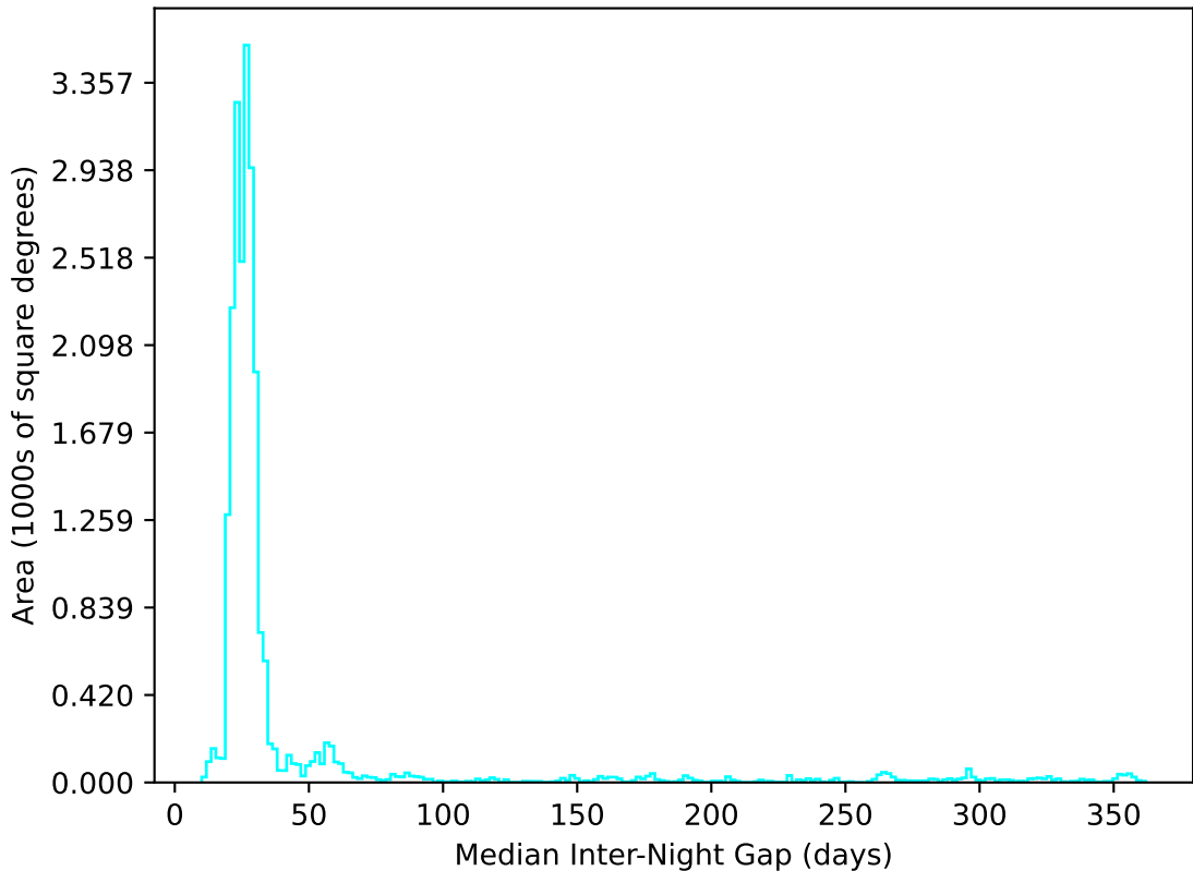
weather_cloudso31v3.4_10yrs All sky u band: Median Inter-Night Gap
