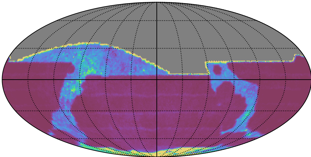
weather_cloudso31v3.4_10yrs All sky r band: Median Inter-Night Gap
