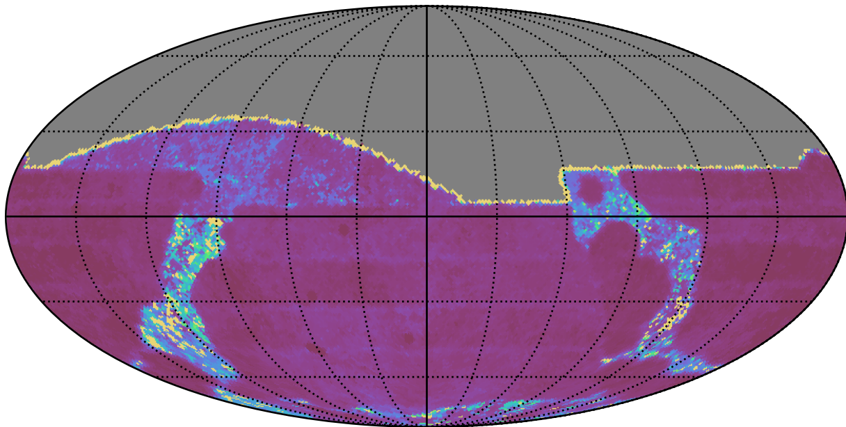
weather_cloudso31v3.4_10yrs All sky g band: Median Inter-Night Gap
