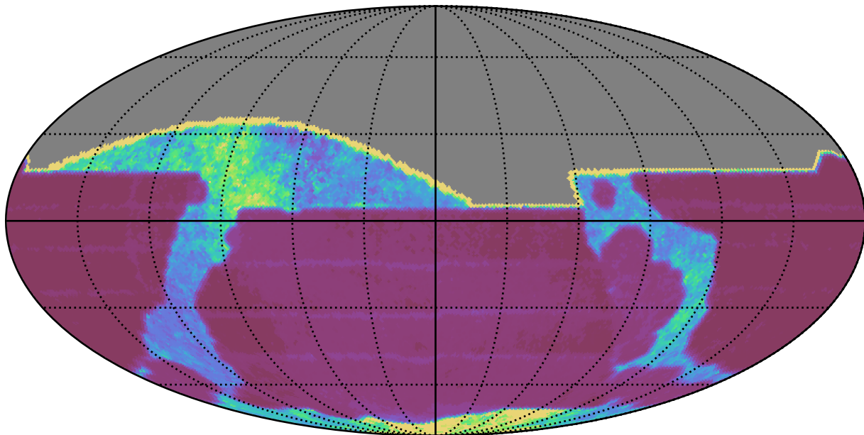
weather_cloudso31v3.4_10yrs All sky all bands: Median Inter-Night Gap
