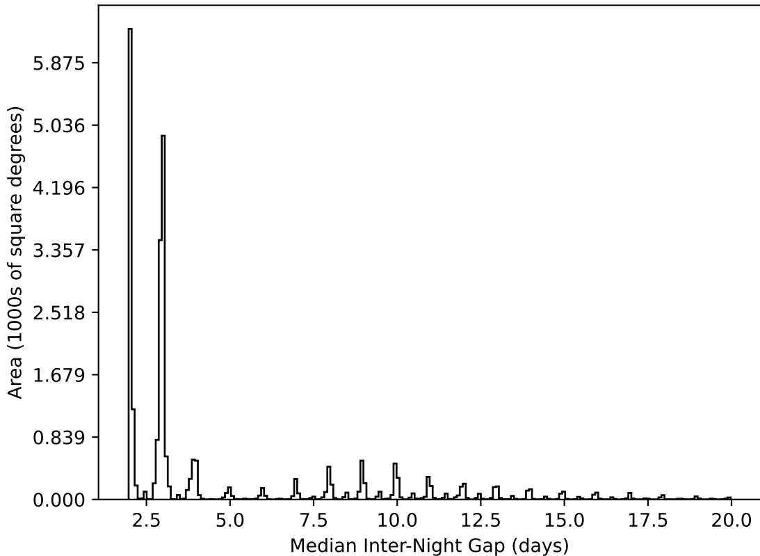
weather_cloudso31v3.4_10yrs All sky all bands: Median Inter-Night Gap
