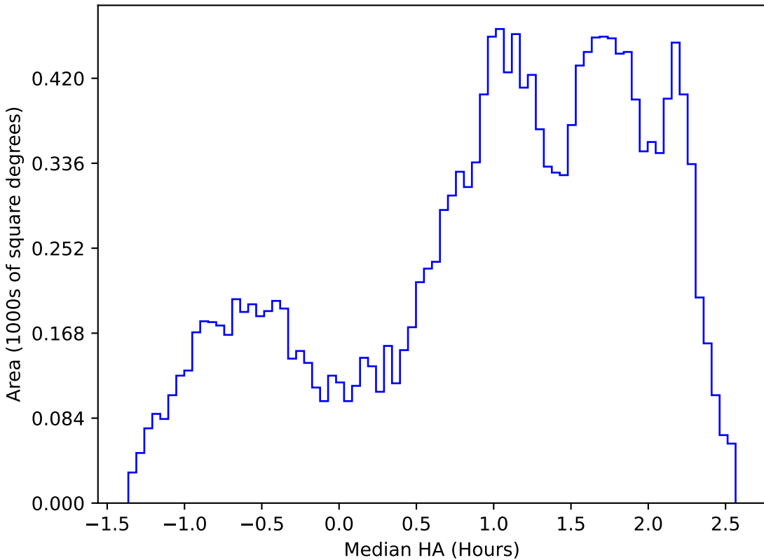
weather_cloudso31v3.4_10yrs WFD z band: Median HA
