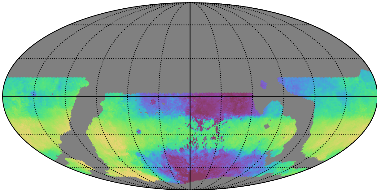
weather_cloudso31v3.4_10yrs WFD y band: Median HA
