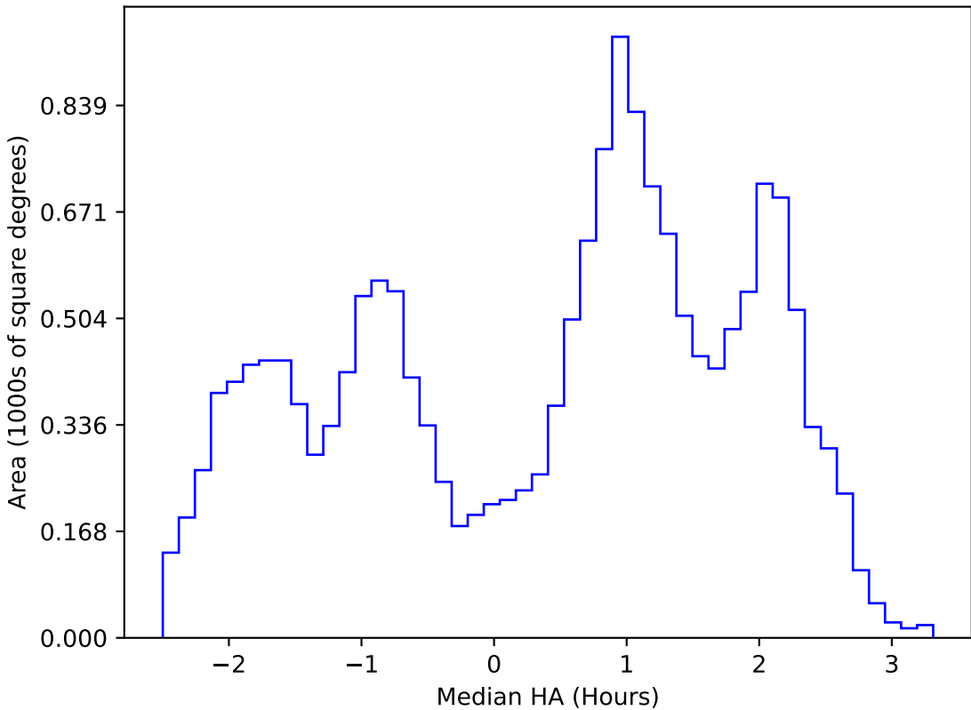
weather_cloudso31v3.4_10yrs WFD u band: Median HA
