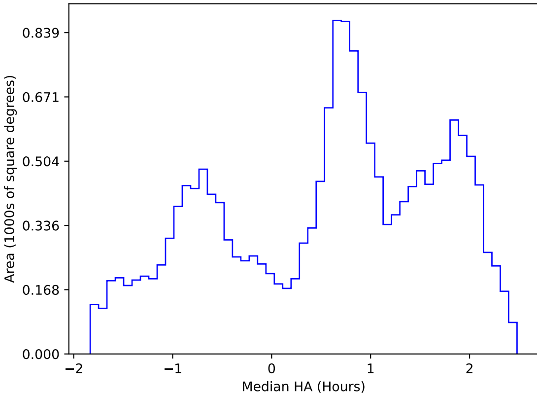
weather_cloudso31v3.4_10yrs WFD r band: Median HA
