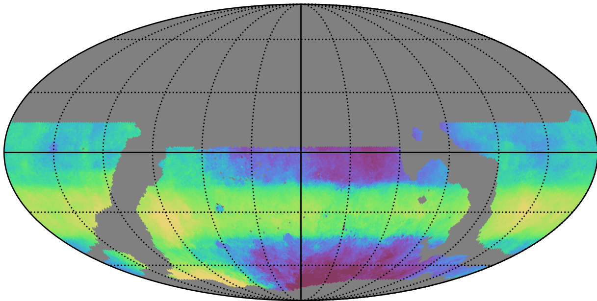
weather_cloudso31v3.4_10yrs WFD i band: Median HA
