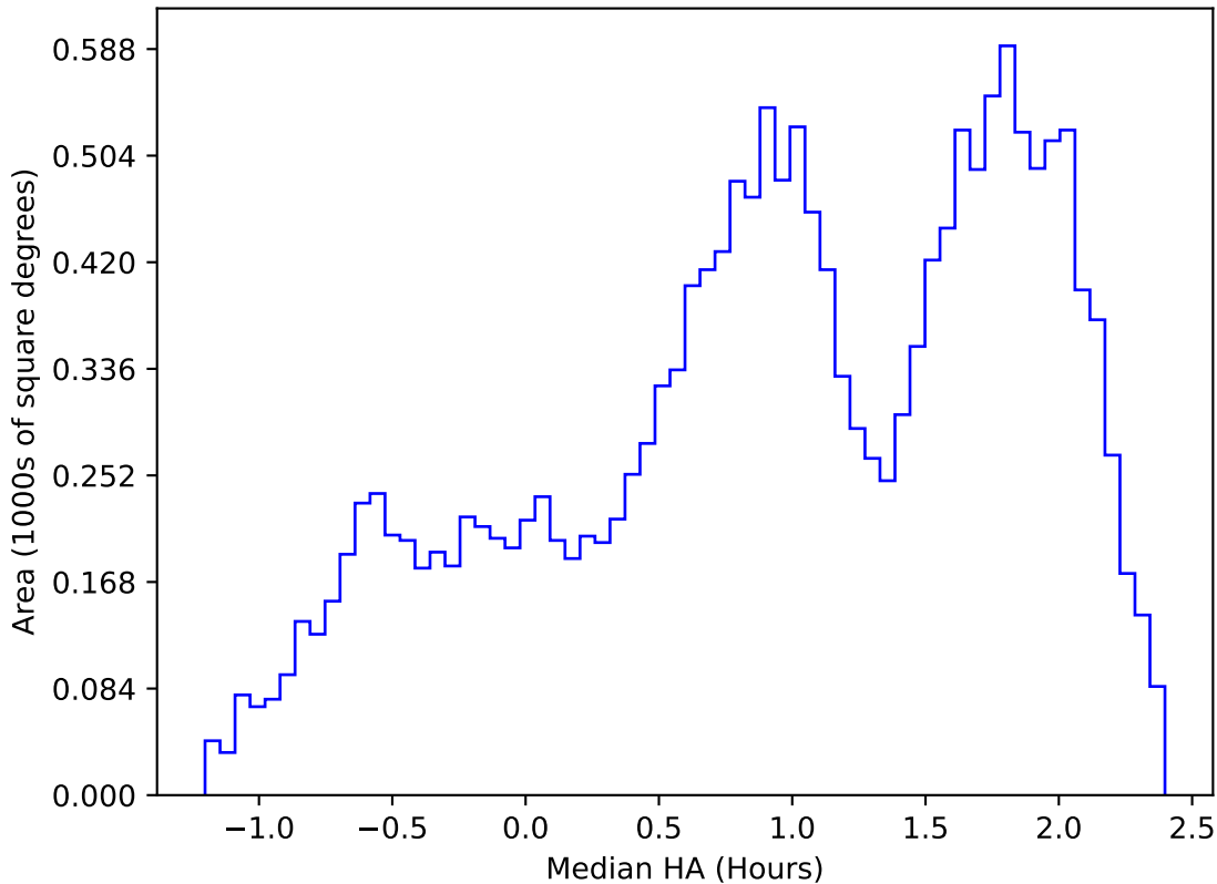
weather_cloudso31v3.4_10yrs WFD i band: Median HA
