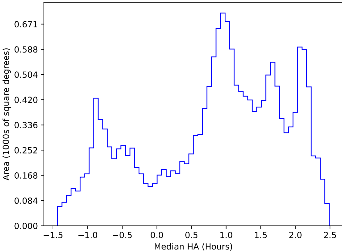
weather_cloudso31v3.4_10yrs WFD all bands: Median HA
