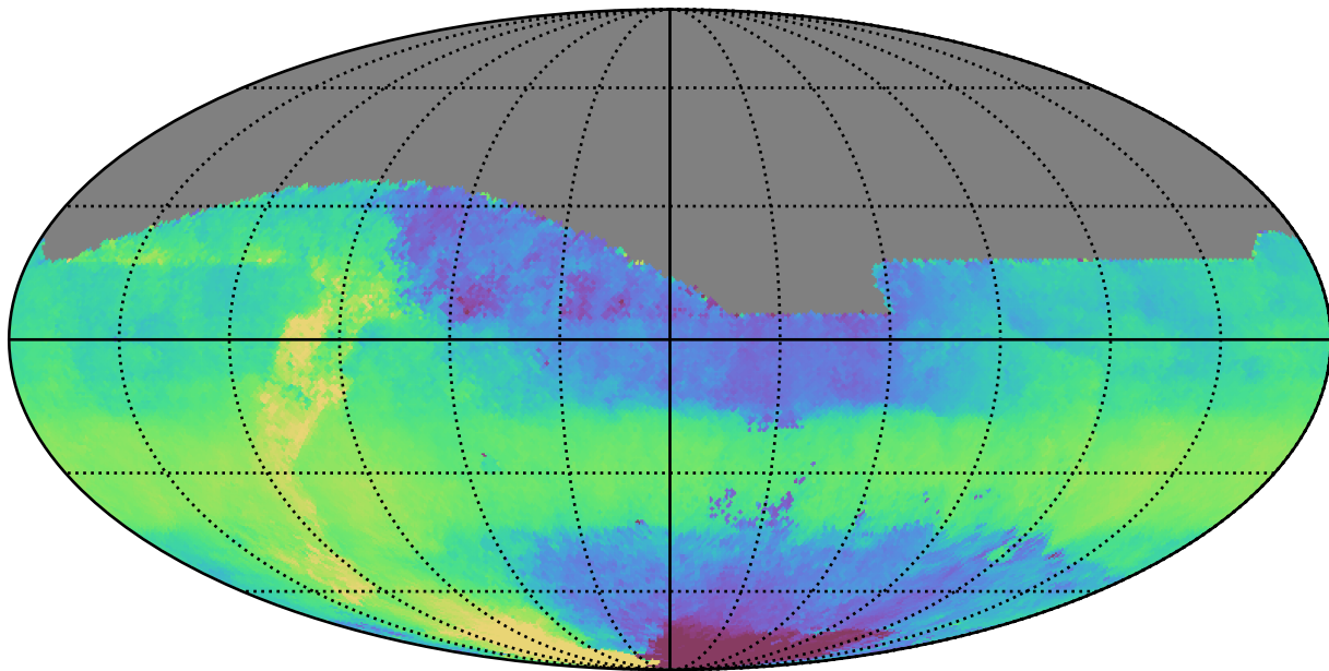
weather_cloudso31v3.4_10yrs All sky z band: Median HA
