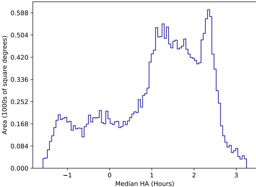
weather_cloudso31v3.4_10yrs All sky y band: Median HA
