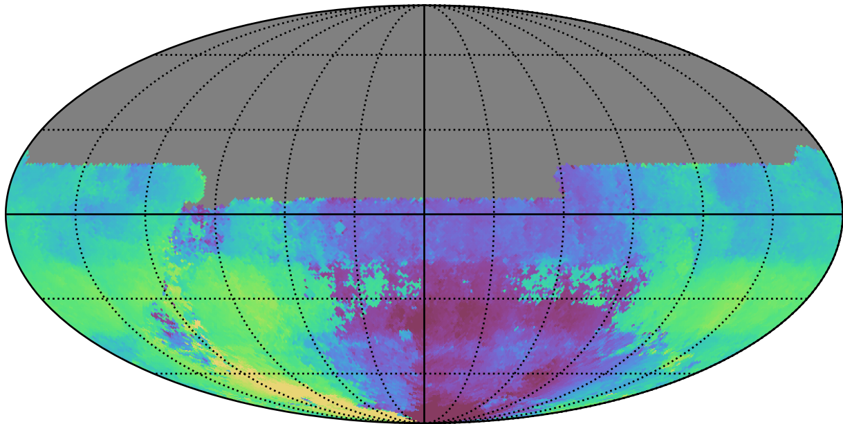
weather_cloudso31v3.4_10yrs All sky u band: Median HA
