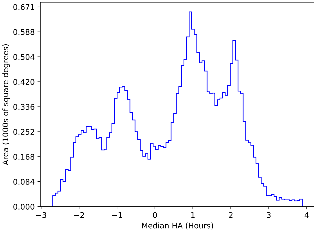
weather_cloudso31v3.4_10yrs All sky u band: Median HA
