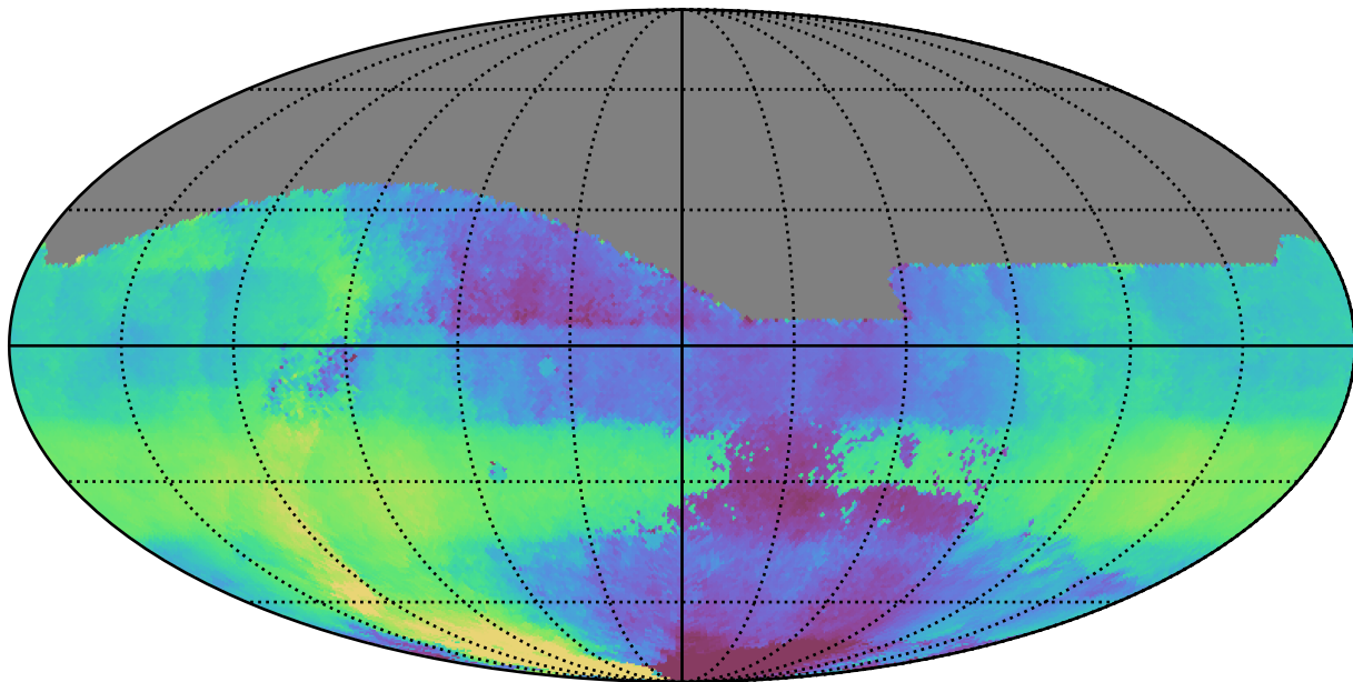
weather_cloudso31v3.4_10yrs All sky r band: Median HA
