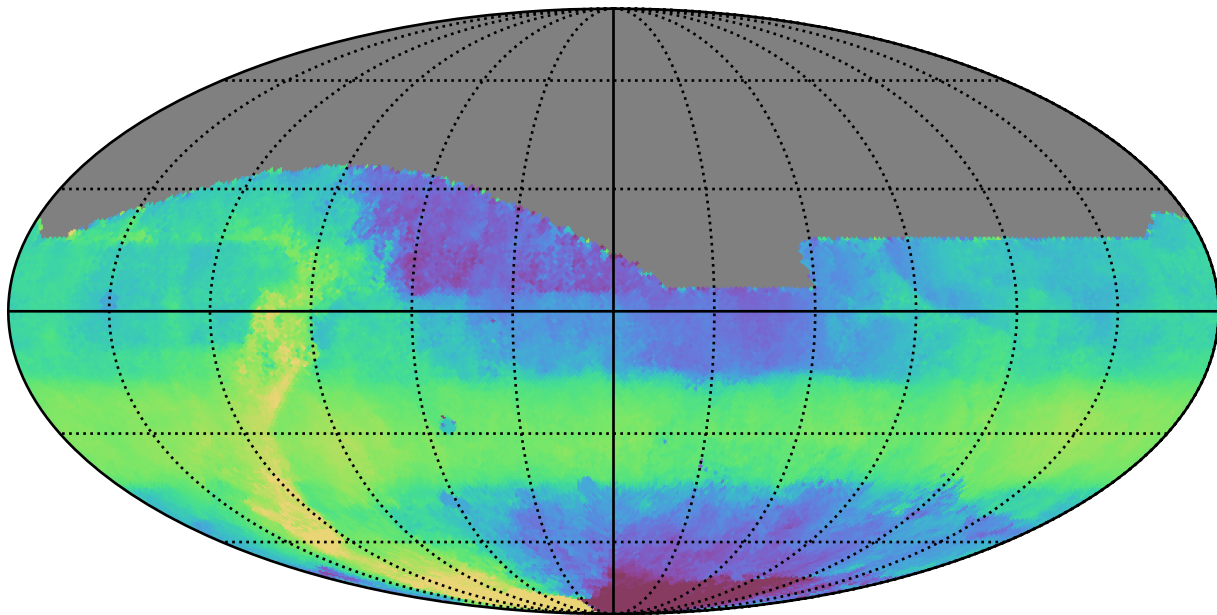
weather_cloudso31v3.4_10yrs All sky i band: Median HA
