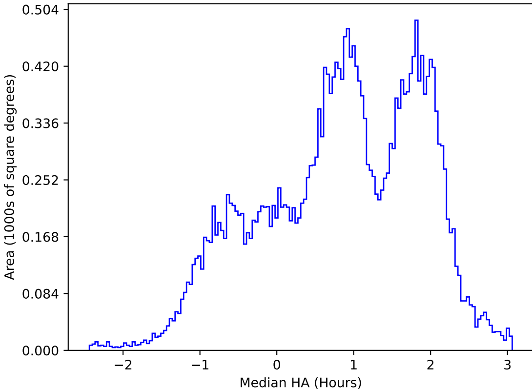
weather_cloudso31v3.4_10yrs All sky i band: Median HA
