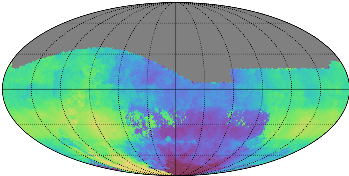
weather_cloudso31v3.4_10yrs All sky g band: Median HA
